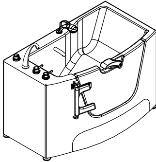
PERSPECTIVE VIEW - N.T.S. MODEL SHOWN HERE AS: LEFT SEAT RIGHT DRAIN (LEFT HAND MODEL SHOWN)
